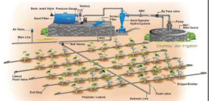
Drip Irrigation System Design Layout
